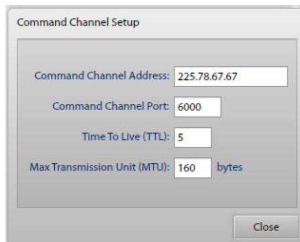
Figure 12. Command Channel Setup dialog box
