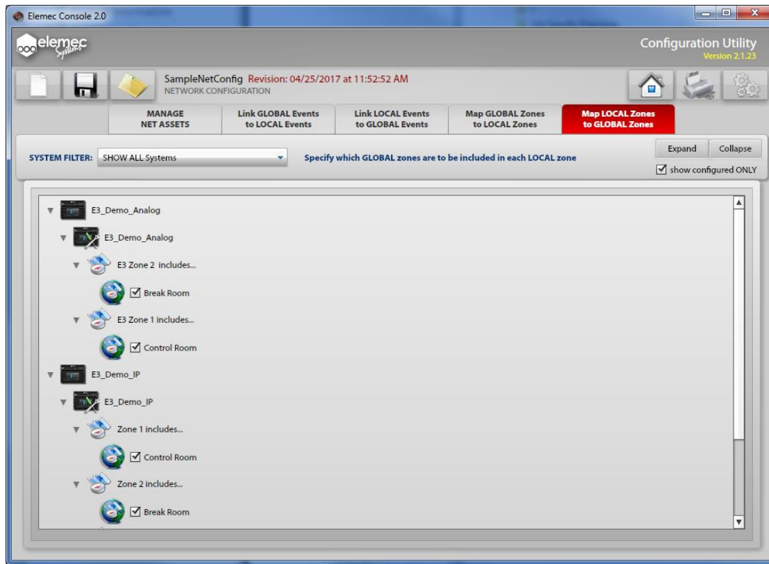
Figure 27. Local Zones Mapped to Global Zones (Configured)
