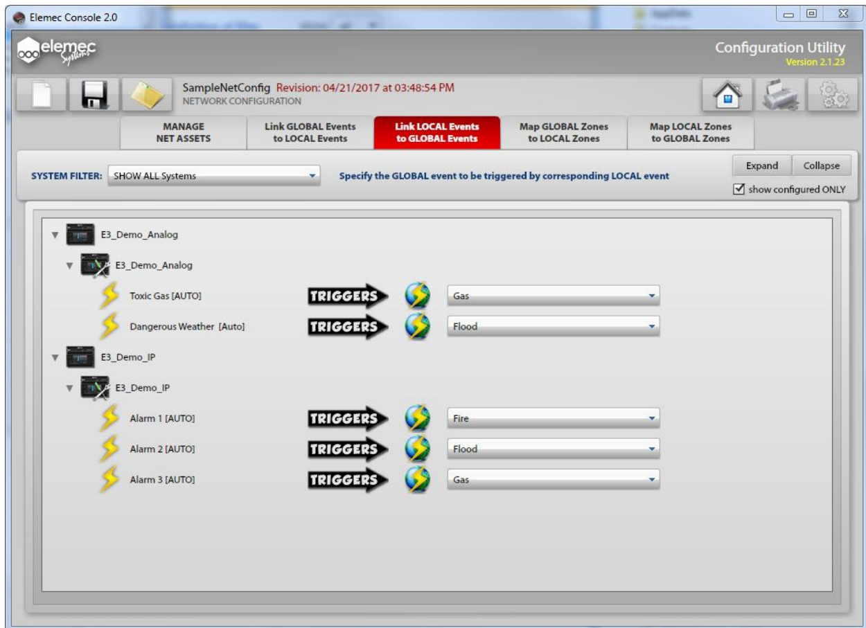
Figure 23. Local Events linked to Global Events (Configured)
