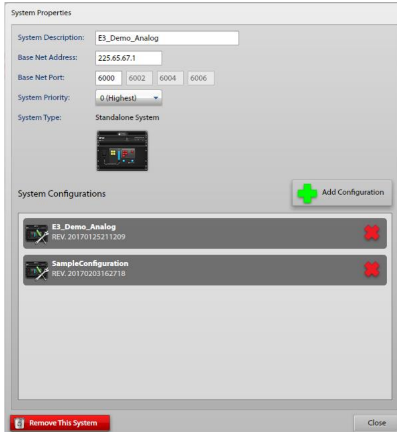
Figure 14. E3 System Properties
