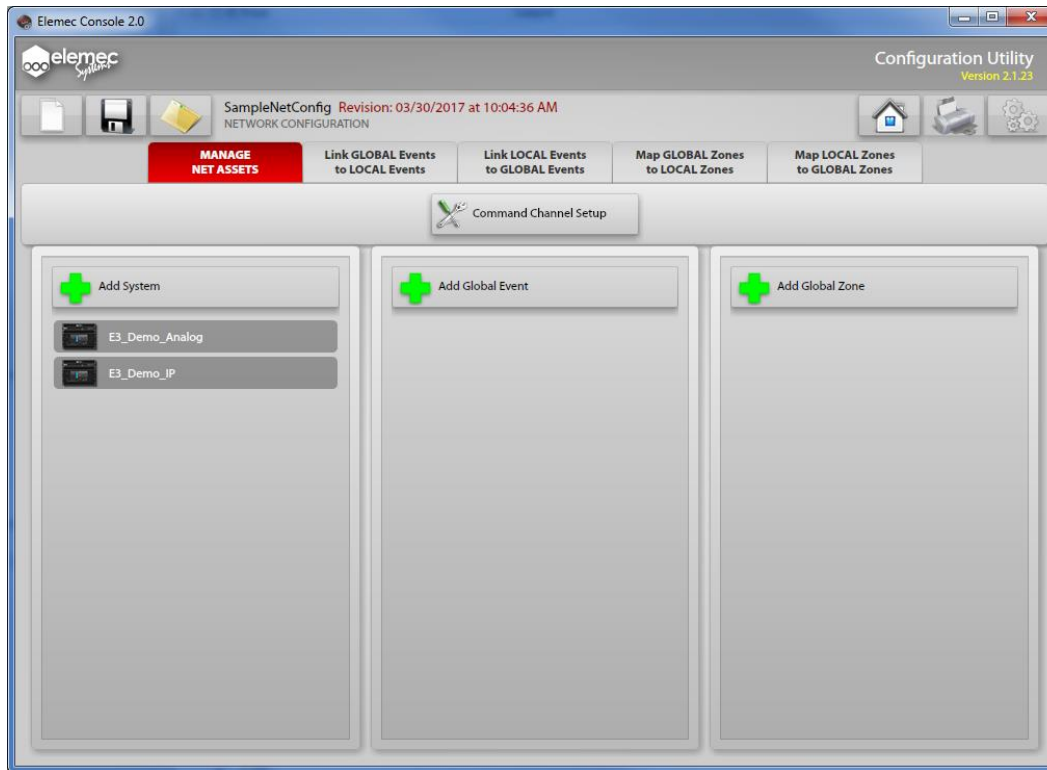
Figure 11. Network Asset Management screen
