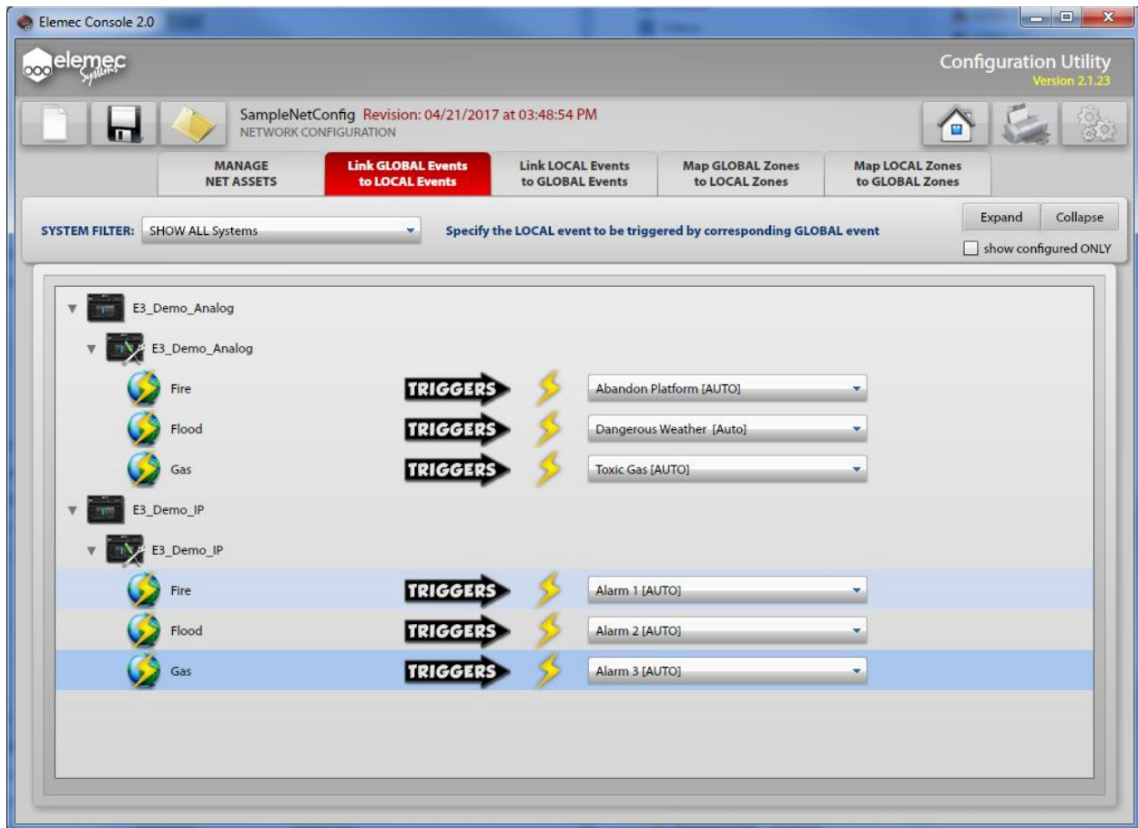
Figure 21. Global Events linked to Local Events
